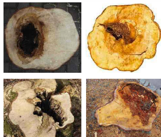
Figure 5. Examples from typical mature urban trees to be inspected in terms of safety: the cross-sections are commonly not circular and the defects are mostly located off-center. Such cross-sections provide many different radius values and many different shell-wall thicknesses (t), often ranging from zero (t=0) to fully wooded (t=Radius). Consequently, there is no typical or average t/R that could be quickly determined at the tree. Furthermore, minimum, maximum, or average t/R values do not represent the load-carrying capacity of such cross-sections. In consequence, the One-Third Rule simply does not apply to these kind of trees.
