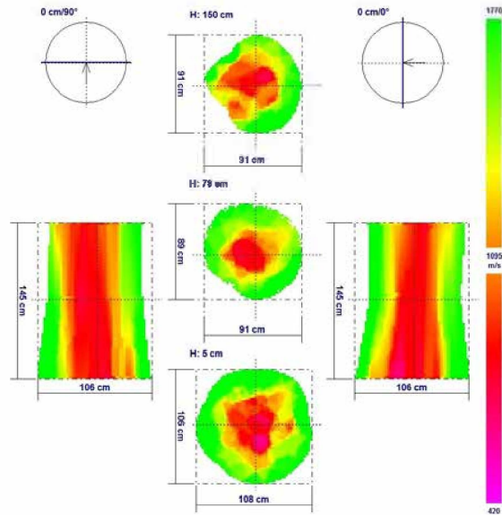
Figure 6. This tree has stood close to a subtropical coastal shore line for more than 100 years. As shown by the sonic tomogram, the stem has been severely damaged and hollow for decades but has survived dozens of hurricanes while young intact trees in the same area broke. This illustrates that the older trees are, the higher their basic safety and the more decay they can tolerate without being significantly more susceptible to breakage.
