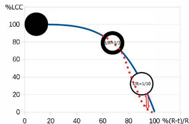
Figure 3. The blue line in this graph shows how the relative load-carrying capacity (% LCC) of a cross-section as represented by the “section-modulus” depends on the ratio of shell-wall thickness divided by the radius. Starting at top left with an intact cross-section, the load-carrying capacity is 100%. Going right, the centrally located void gets bigger and the curve shows how this impacts LCC.
