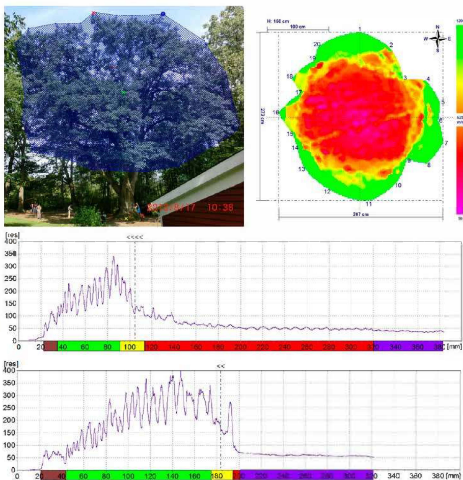
Figure 2. This mature oak tree ( Quercus rubra ) has a diameter at breast height of more than 2.5 meters (8.2 feet). As can be seen by the sonic tomograph (Rinn 1999, 2014b) and the resistance drilling profiles (Rinn 1988, 1990, 2016), the intact outer shell wall ranges from a few to approximately 30 cm (12 inches). The average shell-wall thickness is less than 25 cm (10 inches), which means t/R < 1/5 ( < 1/3 ). This tree is standing despite heavy defects, being hollow for decades, and achieving a height of more than 25 m (75 feet). Arborists strictly applying the One-Third Rule as commonly understood usually condemn such trees as being unsafe or tend to recommend strong pruning and even cabling. However, often there is no need for that—and heavy reductions can significantly contribute to an accelerated spread of internal fungal decay (Rayner & Boddy 1983). Applying the tree-safety concept presented in this article leads to different conclusions for such mature trees and mostly results in nothing to be done or just pruning the crown symmetrically in order to prevent wind-induced torsional loads.
